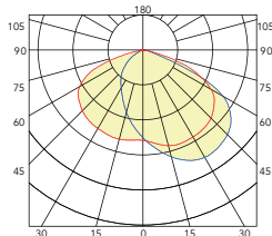
Large size Luminous Intensity Distribution Curve
